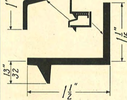
SECTION 318 TOP RAIL OF ALL VENTILATORS
