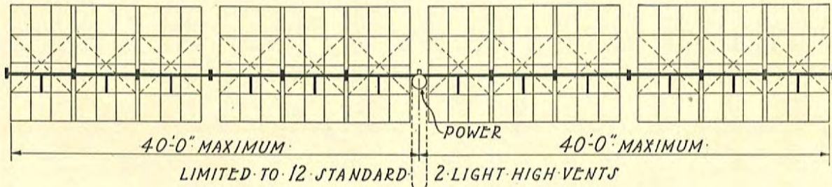
TYPICAL ELEVATION
