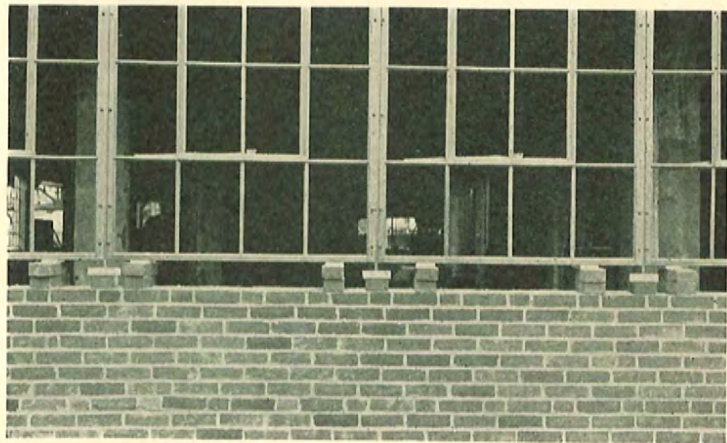
Showing method of supporting windows by blocks or bricks until wedged and bolted.
