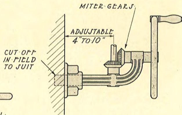
ALTERNATE HANDWHEEL CONTROL
