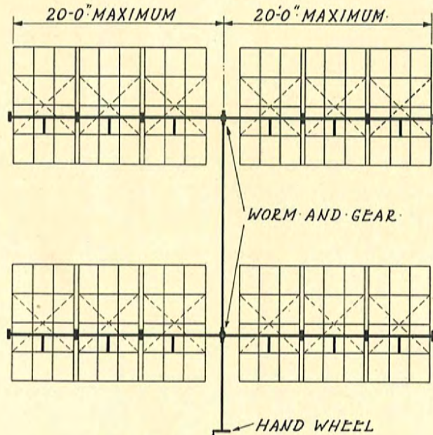
TYPICAL ELEVATION
