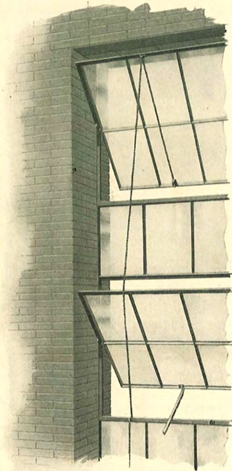
View showing two ventilators in a unit, one above the other. The lower ventilator is operated by Lupton Stay Bar, the upper by Spring Catch and Chain.
