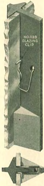
The Standard Lupton Glazing Clip, No. 039, with putty partly broken away.
