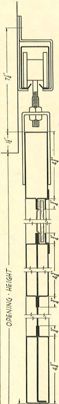
VERTICAL SECTION for SINGLE & DOUBLE DOORS
