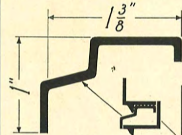
SECTION 335 WEATHERING MEMBER USED WHEN VENTILATOR OCCURS AT TOP OF WINDOW
