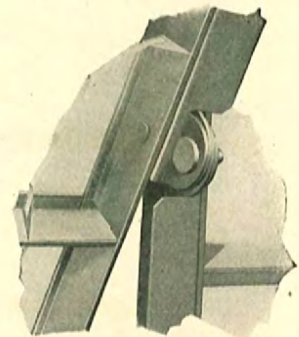
The Lupton Ventilator Hinge. It cannot get out of alignment, being integral with the weathering.
