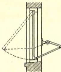
TOP HUNG
