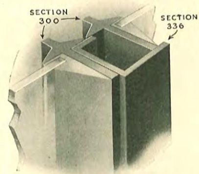
Detail of weathering, showing double contact made by Section 336, and enclosed air space.
