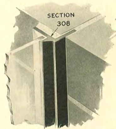
Perspective showing \frac{1}{8} inch lap on flange of window.
