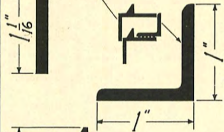
SECTION 103 WEATHERING MEMBER USED WHEN VENTILATOR OCCURS AT BOTTOM OF WINDOW
