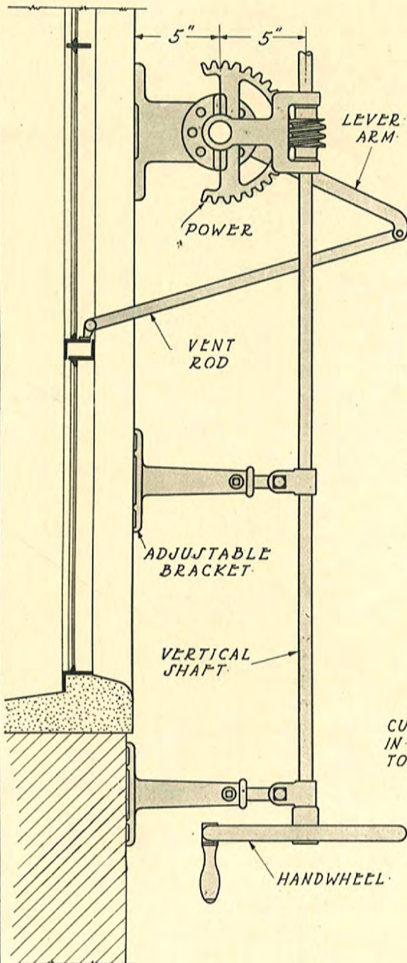
VERTICAL SECTION AT HANDWHEEL CONTROL
